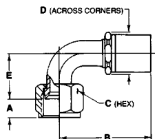
90° ELBOW
