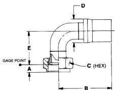
90° ELBOW
